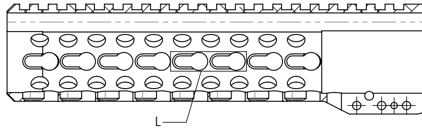
SECTION K-K
