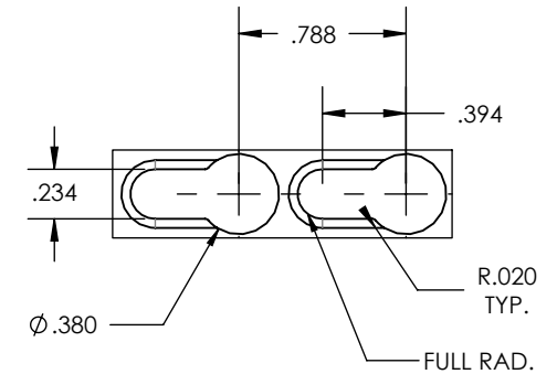
DETAIL L SCALE 1 : 1
