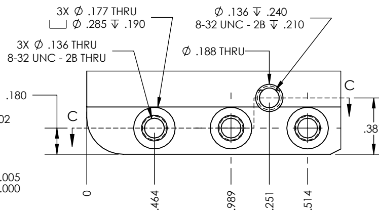
DETAIL B SCALE 1.5 : 1
