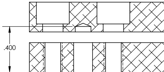
DETAIL E SCALE 2 : 1
