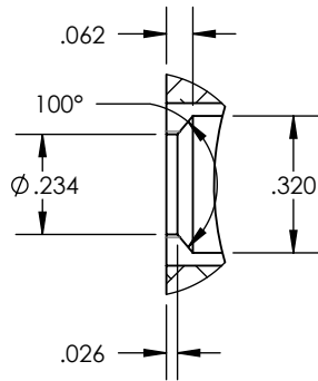
DETAIL M SCALE 2 : 1
